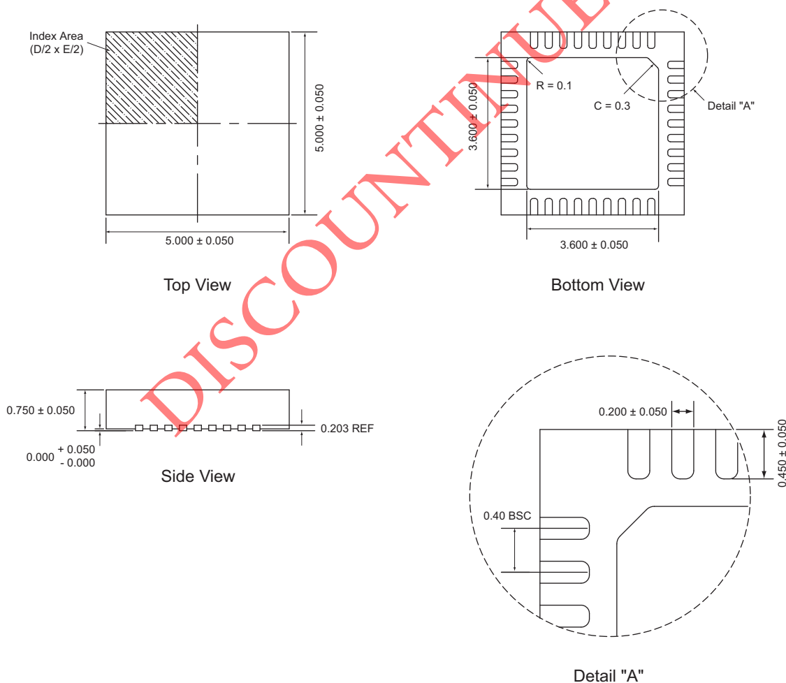
TQFN55-36 3
